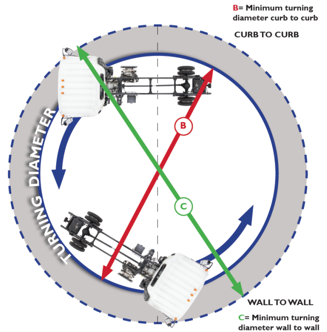
Figure 6: NRR EV Turning Circle Diagram
