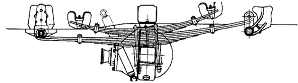
Figure 9: NRR EV Rear Suspension
