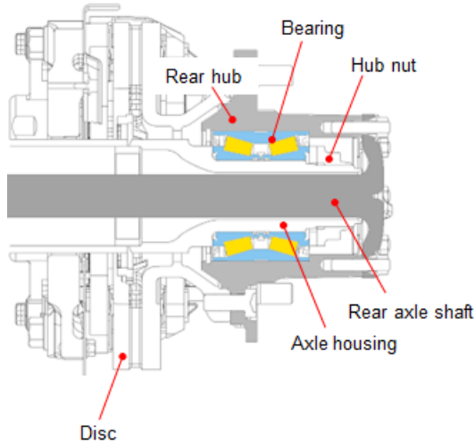
Figure 8: NRR EV Rear Axle
