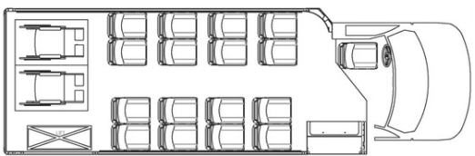
16 Passenger + 2 Wheelchairs + Driver
