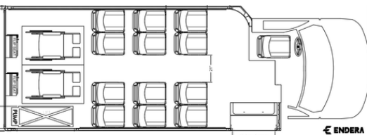
12 Passengers + Two Wheelchairs Plus Driver
