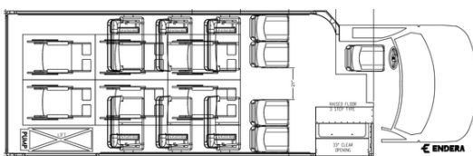
6 Wheelchairs + 4 Passengers or 16 + 2 Plus Driver
